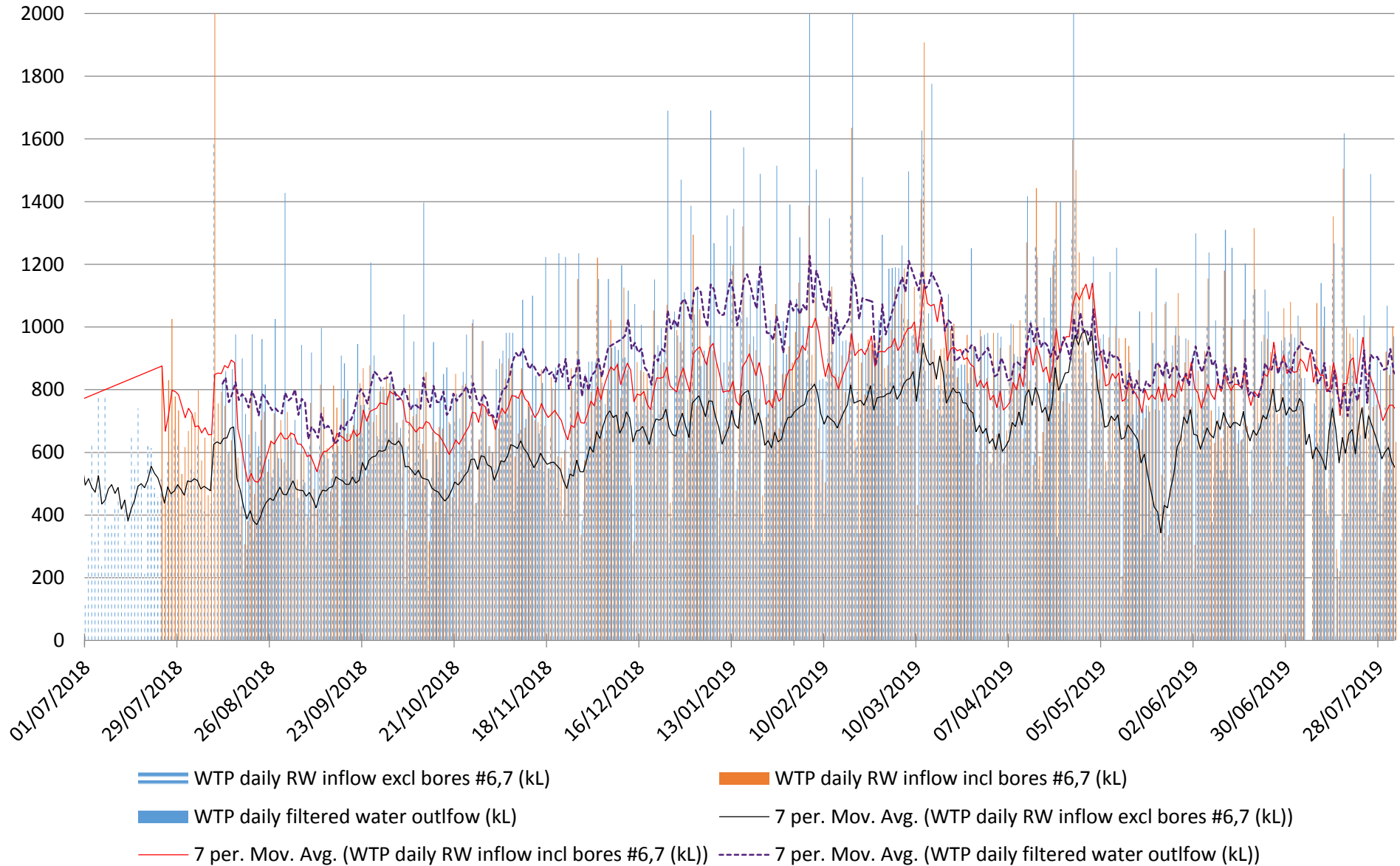
Coonabarabran WTP daily raw water (RW) inflow and filtered water outflow (in kL)
